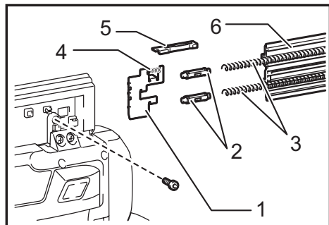
► 1. Pusher 2. Sleeve 3. Spring (large) 4. Spring (small) 5. Stopper 6. Slide door
